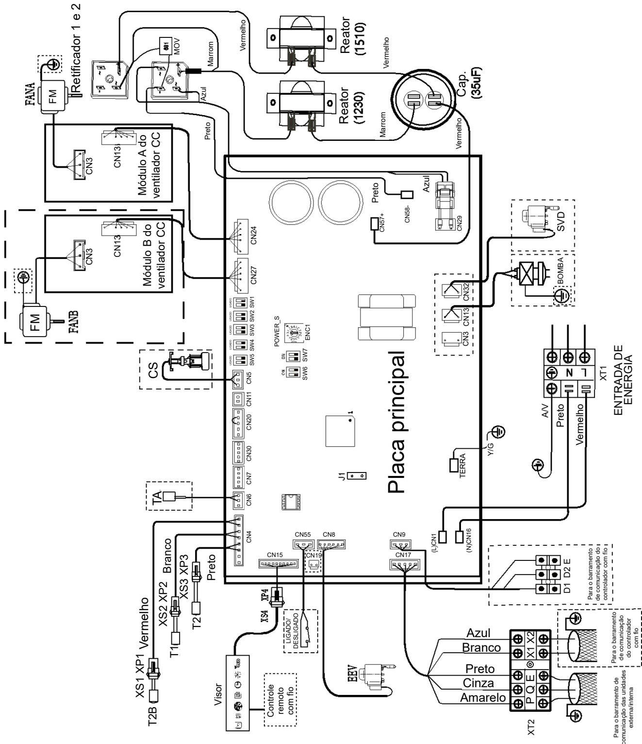
Figura 7: Diagrama elétrico do 4TVF0068(85-95)EF000AAFADHN1
